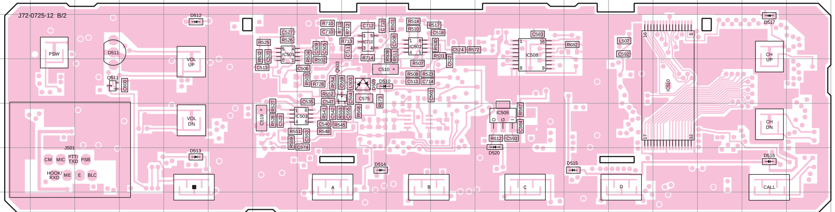
TX-RX UNIT (X57-6152-XX) (B/2) -70 : E -71 : E4 Component side view (J72-0725-12 B/2)
