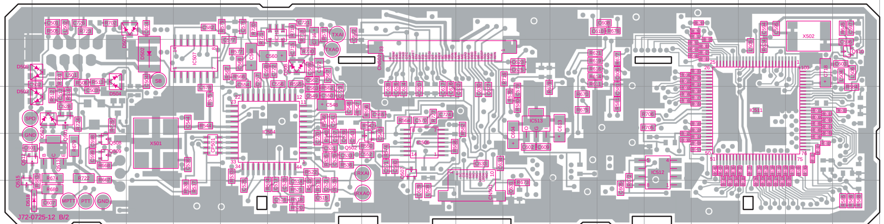
TX-RX UNIT (X57-6152-XX) (B/2) -70 : E -71 : E4 Foil side view (J72-0725-12 B/2)
