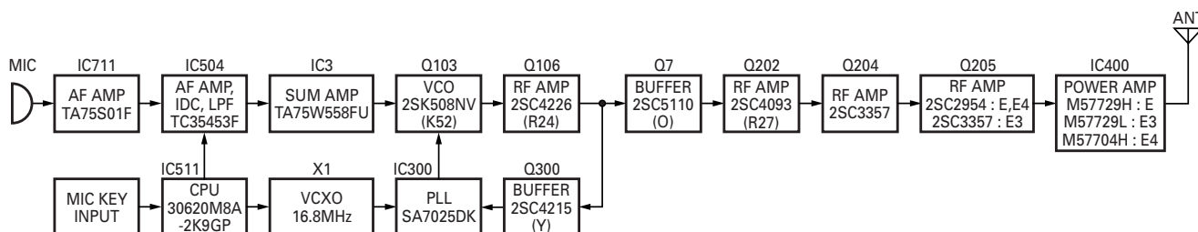
Fig. 6 Transmitter system
